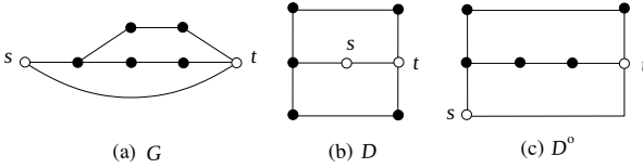
Fig. 3. (a) A biconnected series-parallel graph G , (b) an optimal drawing D , and (c) an outer drawing D^o
