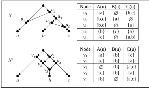
Fig. 2. Two networks N and N' whose tripartition-based distance tri(N, N') = 0.7
