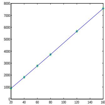
Fig. 2. The X-axis is the number of agents. The Y-axis is the number of running steps. The number of commodities is fixed to 50.
