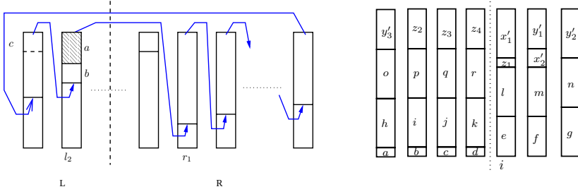
Fig. 3. The procedure of exchange items in Algorithm IMPROVEDALG
