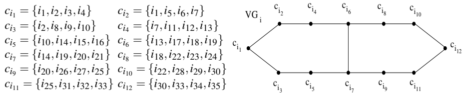
Fig. 3. A vertex gadget and its 2-components
