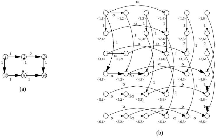
Fig. 3. (a) An acyclic graph G . (b) Graph \bar{G} of (a)
