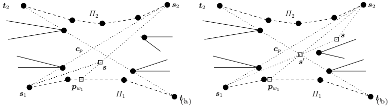
Fig. 4. Agents can start along their shortest path if both see an additional point s
