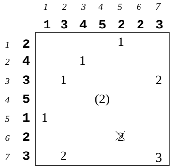
Fig. 1. With two sequences 2435123 and 1345223, the ranks of the critical matches, before and after match (4, 4) is considered, are shown. Match (4, 4) finds two dominating matches (2, 3) and (3, 2), which are with the largest rank 1. Then match (4, 4) has rank 2 and match (6, 5) becomes non-critical.
