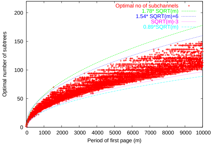
Fig. 3. The optimal number of subtrees ( s_{\text{opt}} ) vs. the period ( m ) of the first page. The actual optima are plotted as data points.
