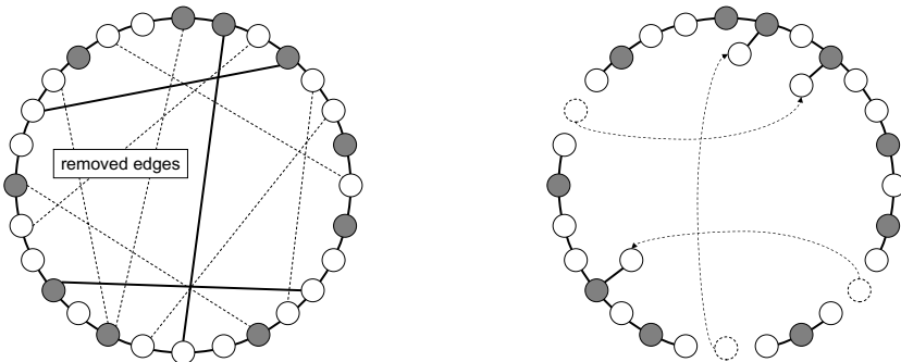
(a) An example of graph G' . (b) An example of graph G'' .
